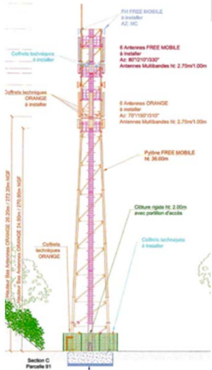
Antenne relais Free Mobile
